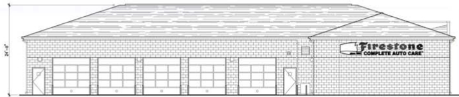
Rear Elevation
